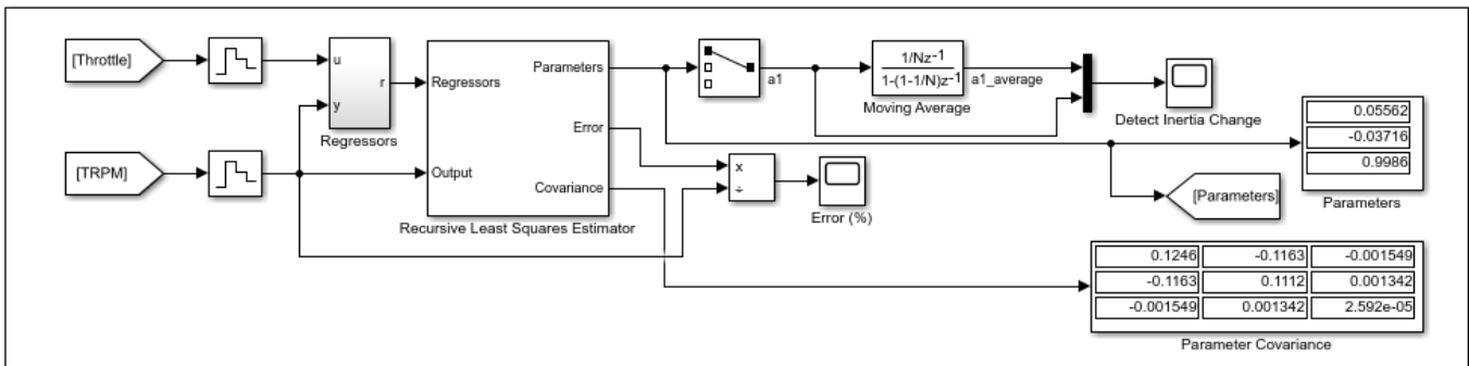
Recursive Estimator
