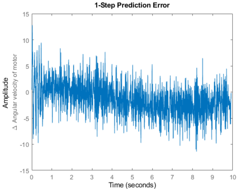
Figure 6: Prediction errors of the estimated robot arm model.
