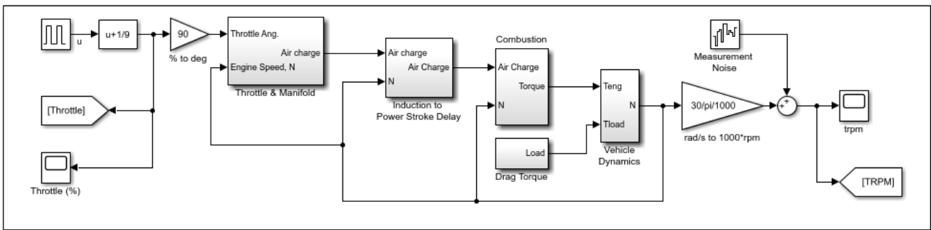
Engine Model
