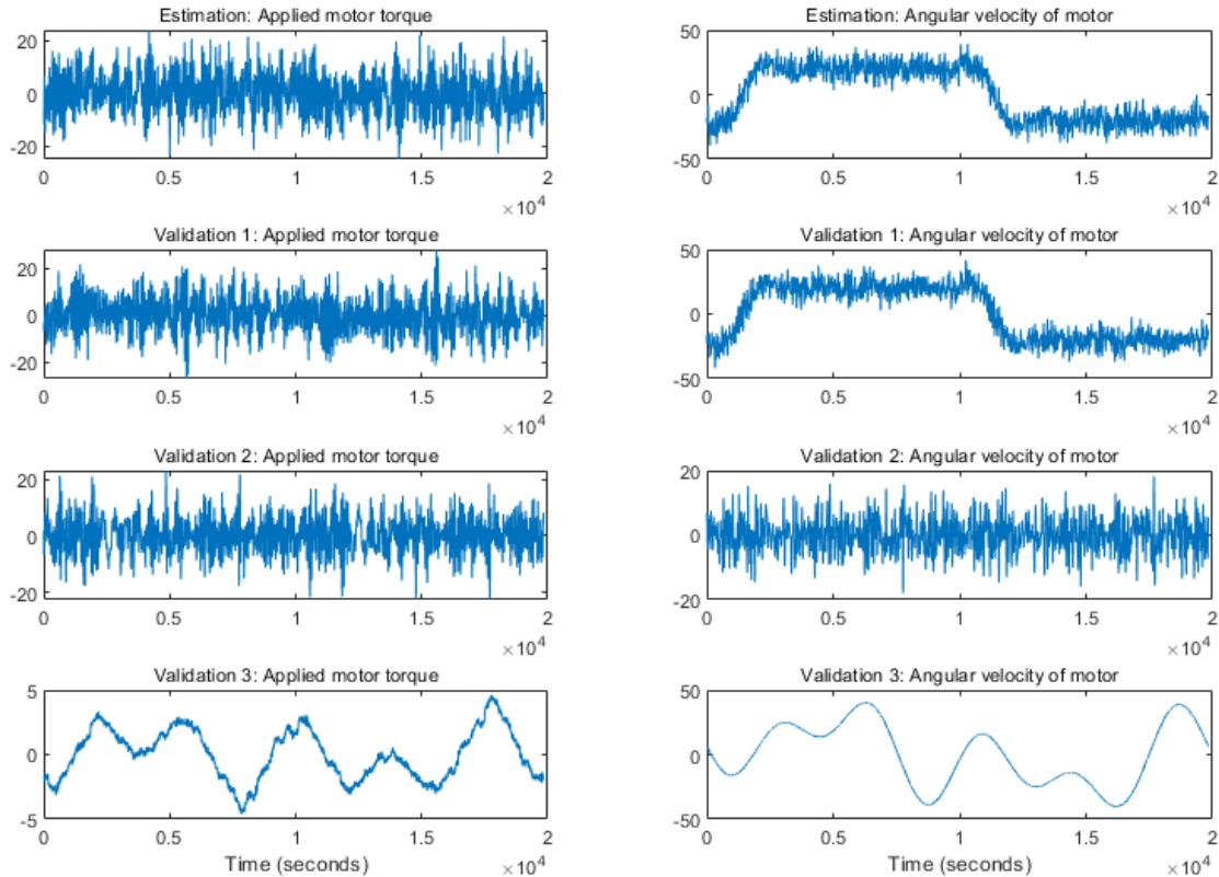
Figure 2: Measured input-output data of an experimental robot arm.
